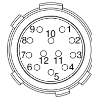
HR10A-10P-12S 12-polig Buchse
